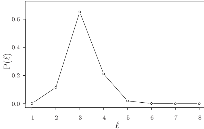
Figure 3. The distance distribution P(\ell) in the largest connected component of the FP5 is shown. The mean value is 3.14 and the farthest pair of nodes in the graph is separated by only 8 edges.
