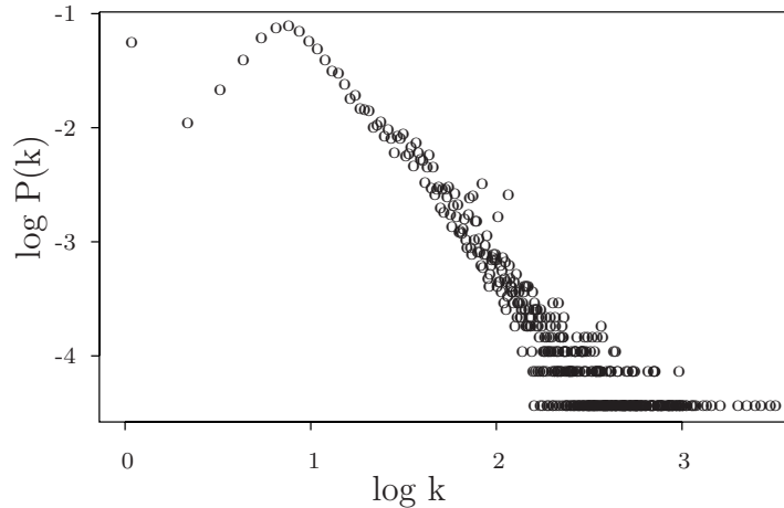
Figure 1. This figure depicts the degree distribution of the FP5 network on a log – log scale. The average degree is k = 26.1 and the maximum degree is a striking k_{max} = 2,784 . The points lying on the right of the maximum fit well a power–law, P(k) \sim k^{-\gamma} , where \gamma = 1.86 \pm 0.02 with coefficient of determination R^2 = 0.85 .
