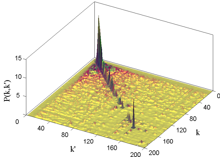
Figure 5. Joint degree–degree distribution of the FP5 network. The X and Y axes represent the degrees k and k' and the Z axis gives the corresponding joint degree–degree probability in per mill. The range is limited from 0 to 200 to illustrate a clearer picture. The distribution peaks on the line k = k' which implies that the FP5 shows assortative mixing.
