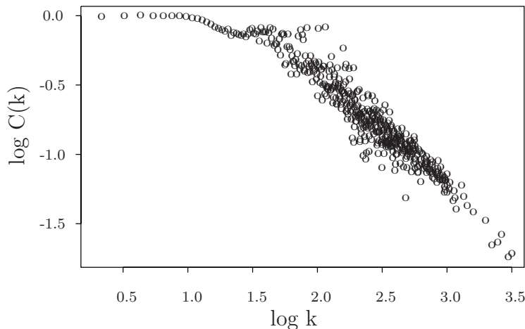
Figure 2. In this figure the clustering coefficient as a function of k in a log – log plot is shown. After the initial plateau, where C(k) is approximately constant, it decays as a power-law, C(k) \sim k^{-\alpha} , where \alpha = 0.77 \pm 0.01 with R^2 = 0.88 .
