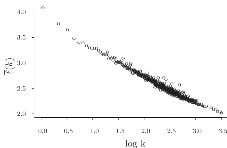
Figure 4. The average distance of a vertex of degree k to all other vertices in the LCC is depicted. It can be seen the logarithmic dependence of the points since it is verified that \bar{\ell}(k) \sim \log k^{-\beta} where \beta = 0.555 \pm 0.004 with R^2 = 0.97 .
