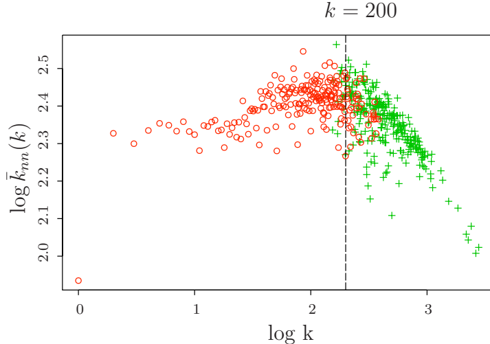
Figure 6. Plot of the mean degree of the nearest neighbors of a vertex of degree k , \bar{k}_{nn}(k) , on a log – log scale. Apparently, the behavior below k \approx 200 is assortative and disassortative for higher degrees. However, only the region with assortative mixing must be considered because over k \approx 200 the finite size of the network is important. If the green crosses are points calculated from only 1 or 2 participants and the rest of the points are red circles, it can be seen that the region with disassortative mixing is essentially made of green crosses.
