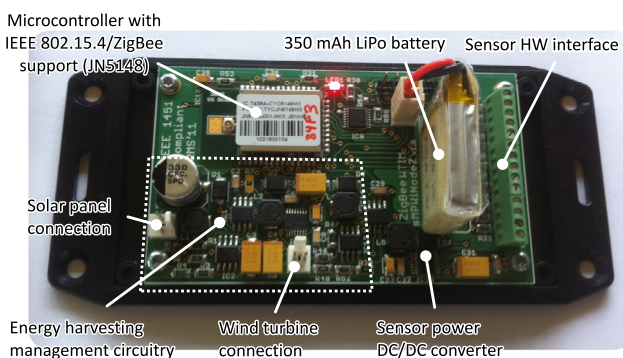
Fig. 4. Picture of the sMPWiNodeZ platform, an IEEE 1451 WTIM.
