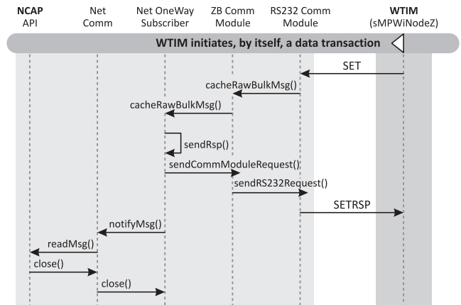
Fig. 14. Operations sequence for receiving incoming data from a sensor attached to WTIM operating in the free running mode. For instance, this sequence is used to retrieve data from a WTIM that is transmitting temperature readings every 5 min.
