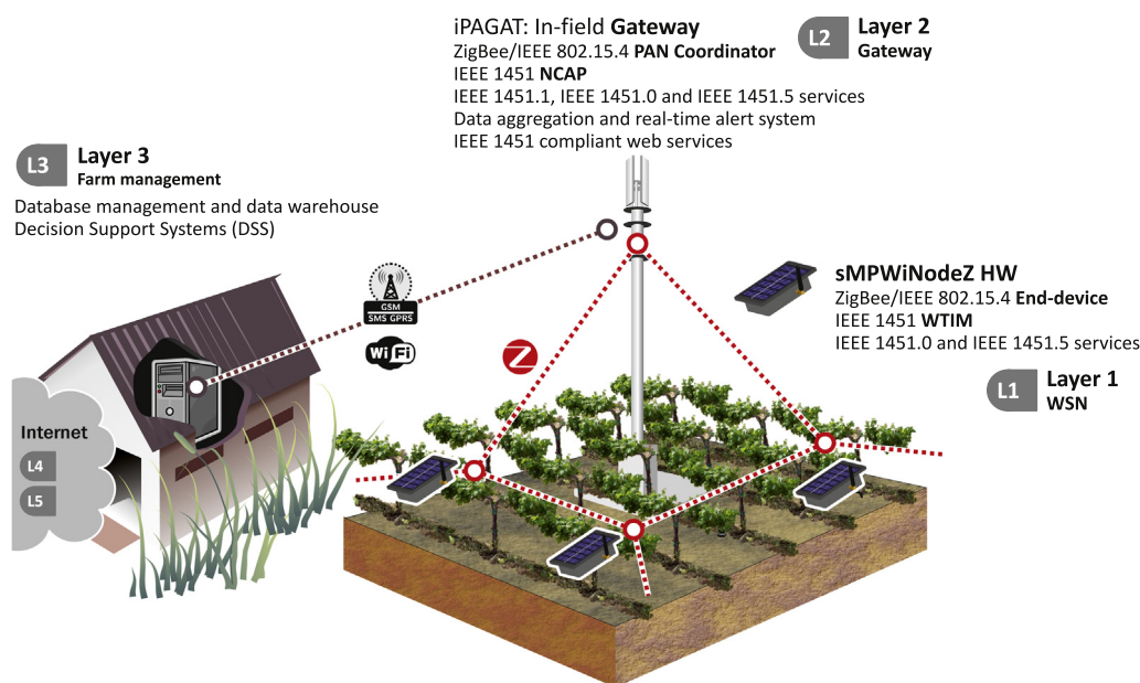
Fig. 2. Illustration of an IEEE 1451 WSN compliant network deployed over a vineyard, emphasizing IEEE 1451 concepts and entities. Each WSN node is a WTIM device while the NCAP acts as a sink node (gateway) to collected data.
