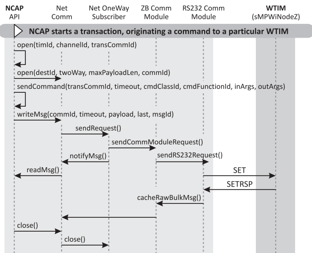
Fig. 13. Operations sequence for sending a command from NCAP to a WTIM accordingly to IEEE 1451.0 specification. This sequence is used, for instance, to program the TC of a WTIM to operate on every sampling period.
