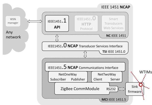
Fig. 7. Functional software architecture of the Java NCAP application embedded in the iPAGAT gateway.
