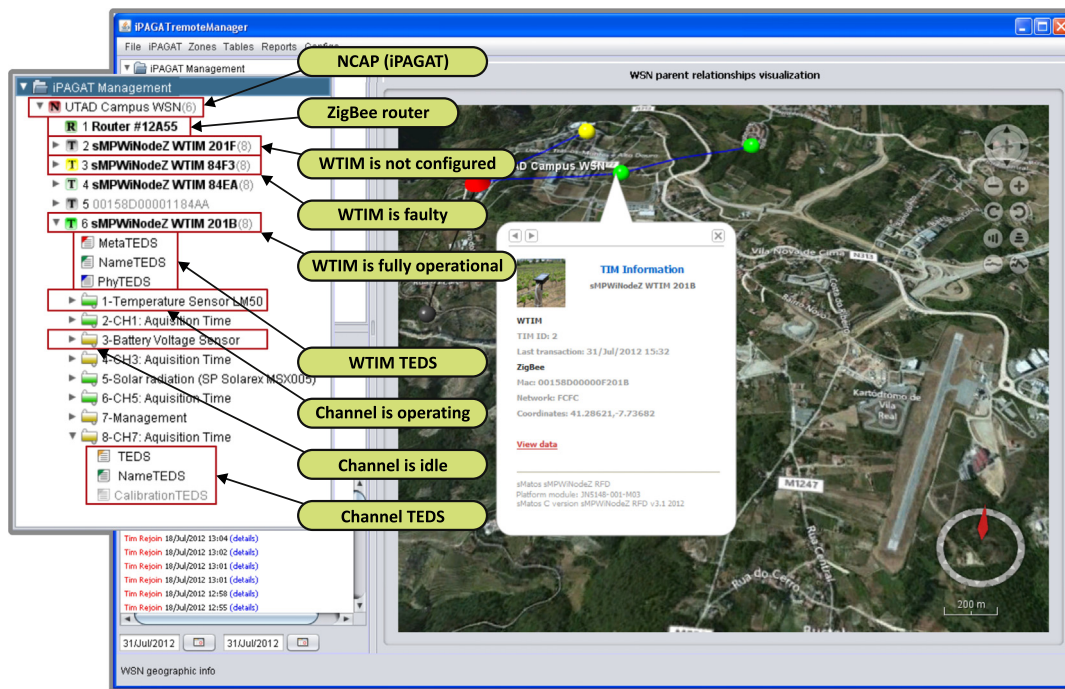
Fig. 10. The Java application that allows the remote management of the iPAGAT gateway and its components. Emphasis on the iPAGAT management tree, illustrating all WTIM details, regarding status, activity and installed TEDS. It makes the complete integration and management of an IEEE 1451 NCAP, as part of the iPAGAT gateway, possible and convenient.
