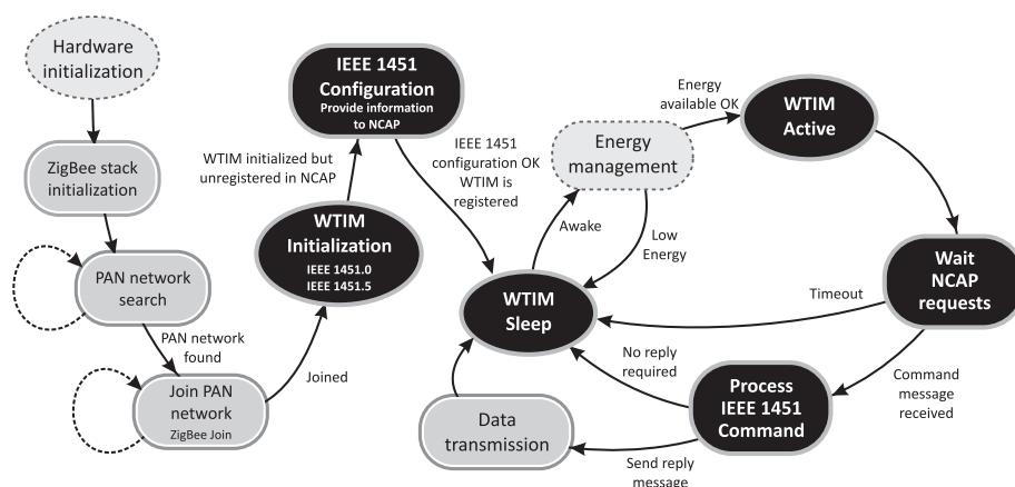
Fig. 6. Simplified representation of the state machine implemented in the sMPWiNodeZ platform. The states WTIM Initialization , WTIM Sleep and WTIMActive are defined by IEEE 1451 and are part of the operation of the WTIM.
