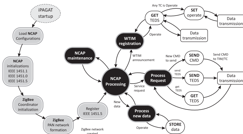
Fig. 8. A simplified state machine representation of the NCAP implementation.
