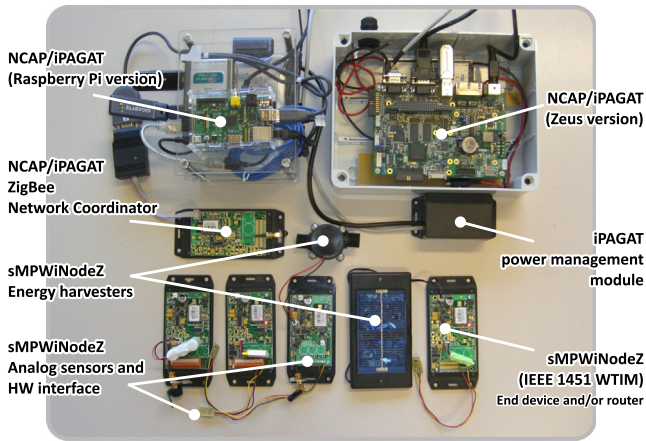
Fig. 9. Devices used in the testing and demonstration WSN. A set of sMPWiNodeZ platforms were configured as IEEE 1451 WTIM. The implementation of the NCAP, as part of a gateway, was initially based on a SBC Zeus and in later stages on a Raspberry Pi (both are shown in the picture).
