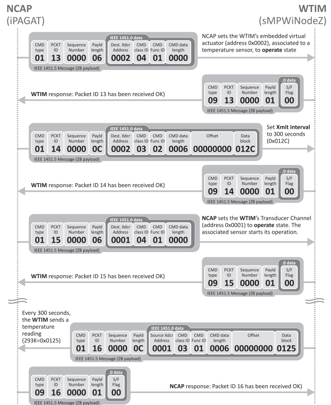
Fig. 15. Command/response pairs and message formats used to describe WTIM's TC configuration operations. The last pair illustrates the transmission of a sensor reading to the NCAP without the need of NCAP polling.
