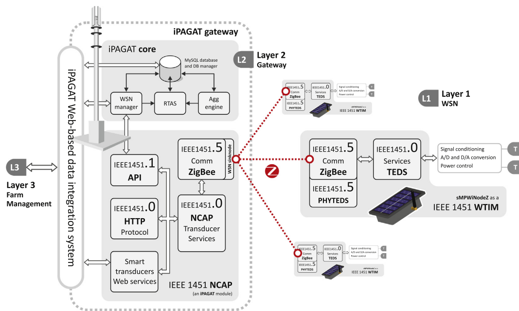
Fig. 3. Functional architecture of the iPAGAT gateway acting as a IEEE 1451 NCAP and related WTIM data acquisition platforms, based on sMPWiNodeZ. iPAGAT core uses IEEE 1451 NCAP services to access WSN data and store it into a local MySQL database using a WSN manager.
