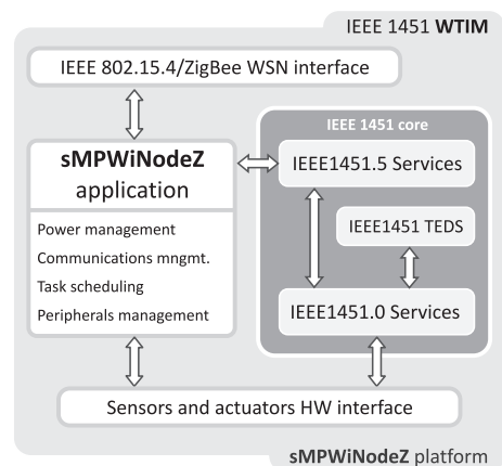
Fig. 5. sMPWiNodeZ platform software structure, which ensures its operation in accordance with IEEE 1451.0 and IEEE 1451.5 IEEE 802.15.4/ZigBee.
