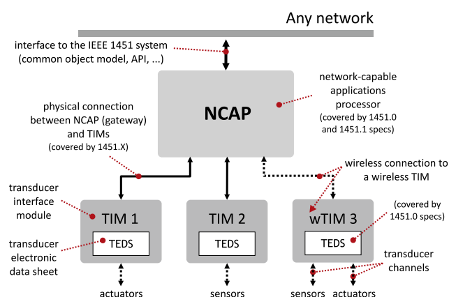
Fig. 1. Under IEEE 1451, a sensor/actuator system is divided into two parts: a Transducer Interface Module (TIM) containing the sensing or actuating element and including signal-conditioning circuits, and a Transducer Electronic Data Sheet (TEDS), digital data that identifies the type of sensor, its calibration information, scale factor, and more. Each TIM is connected to a network-capable applications processor (NCAP), which provides an interface to any network, by a subset of the IEEE 1451 standard.
